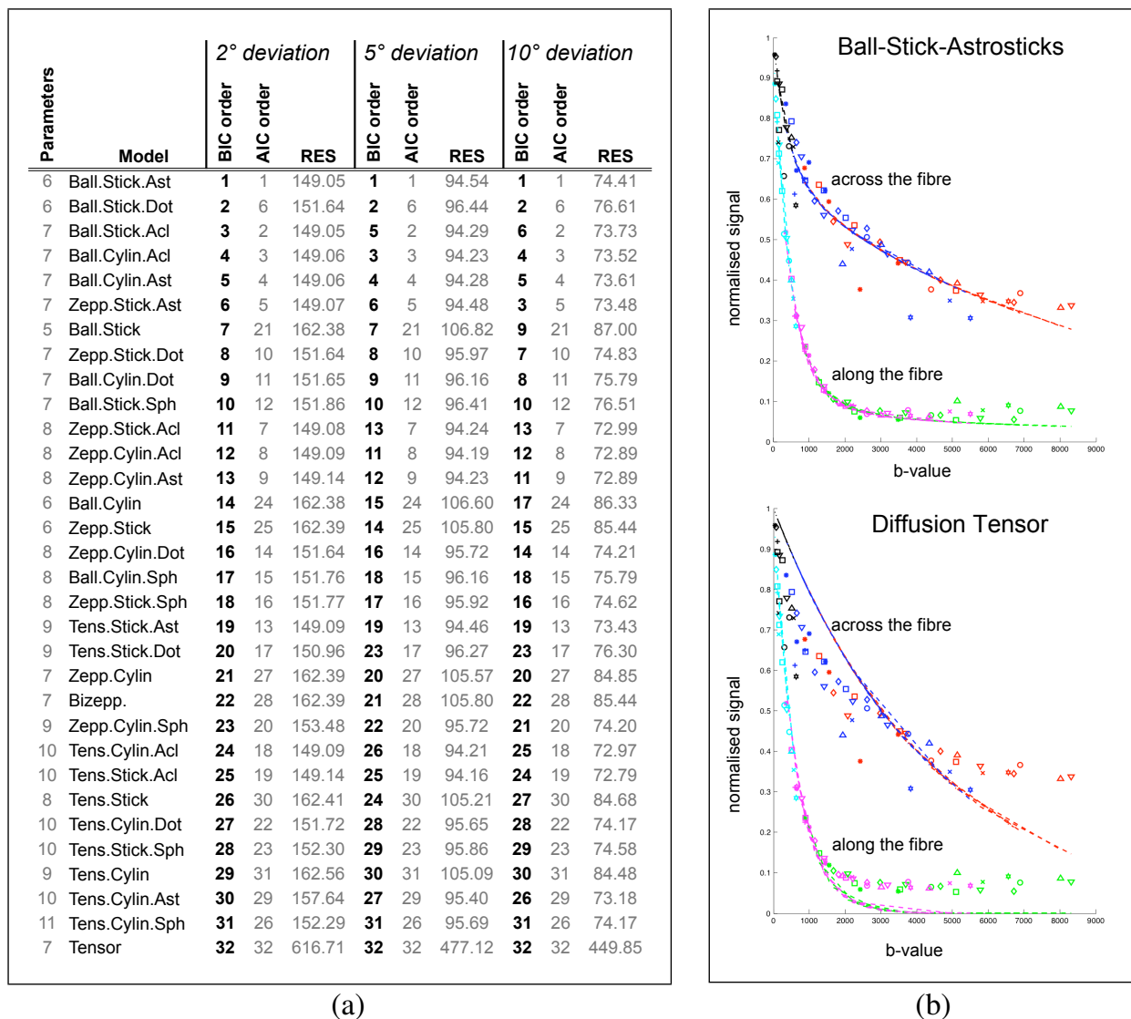
Figure 1: a) Models ranked for the 2 /5 /10 fibre deviation allowances. Adjacent are the raw scores for their respective Objective Function Residue ( RES ). The Ball-Stick-Astrosticks does best across both BIC and AIC , the DT worst. (Abbrev.: Tens.=Tensor; Zepp.=Zeppelin; Cylin.=Cylinder; Ast.=Astrosticks; Acl.=Astrocyinders; Sph.=Sphere). b) Matching the raw signal and the signal synthesized from the model parameters for the 2 threshold data set. The Ball-Stick-Astrosticks model fits the data well; the Tensor (DT) fits poorly.
